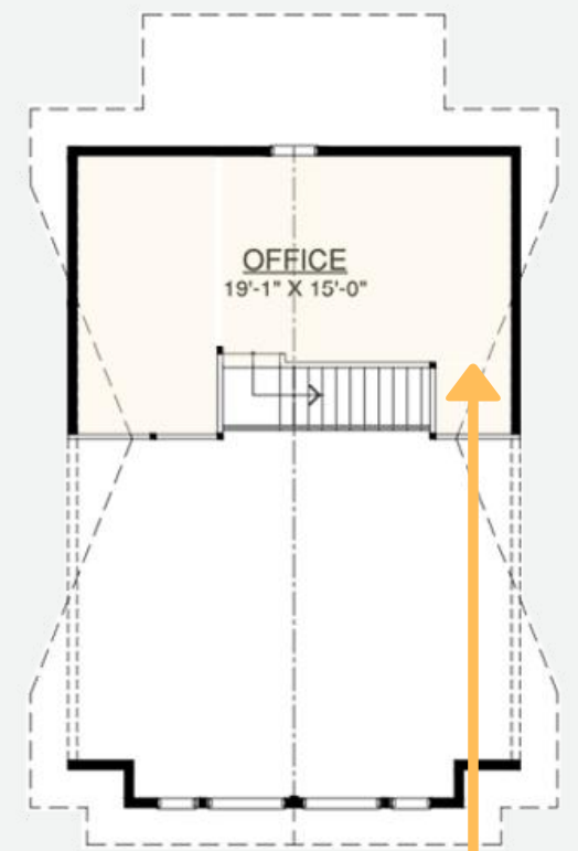
UPPER FLOOR
